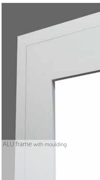
ALU frame (front installation) Lintel + post. Lintel 120 mm (suitable for LHR RM and R40). Lintel 180 mm (suitable for LHR FM). Posts 100 mm.
